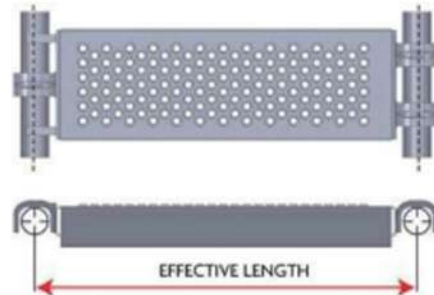
7-9/16" FILLER STEEL PLANK
