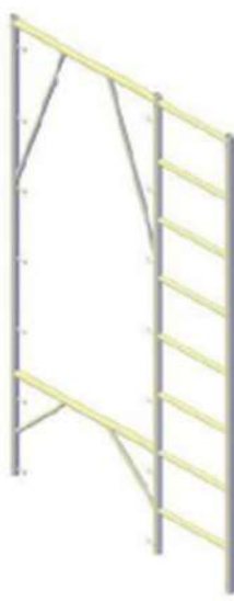
SNAP-ON APT FRAME3'X8'8" W/LADDR
